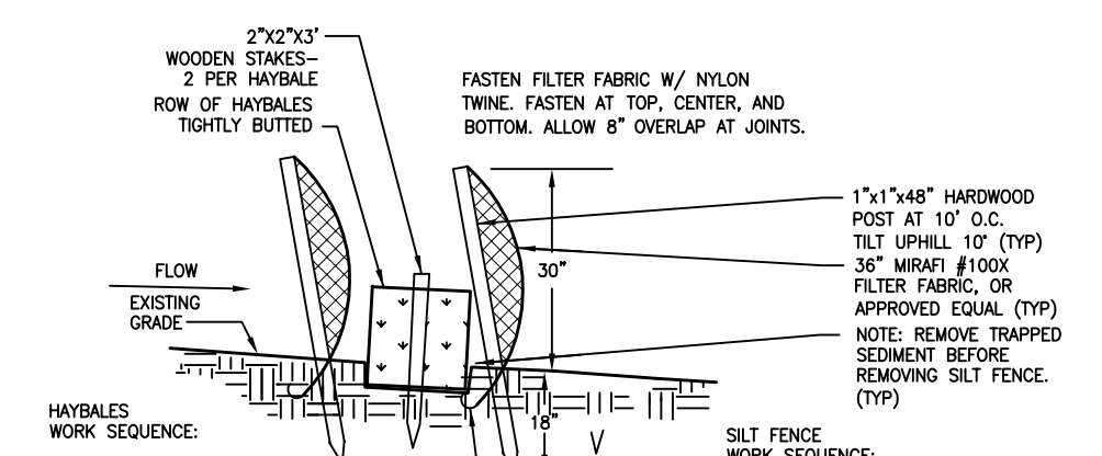
SILT FENCE/HAYBALES/SILT FENCE NOT TO SCALE
