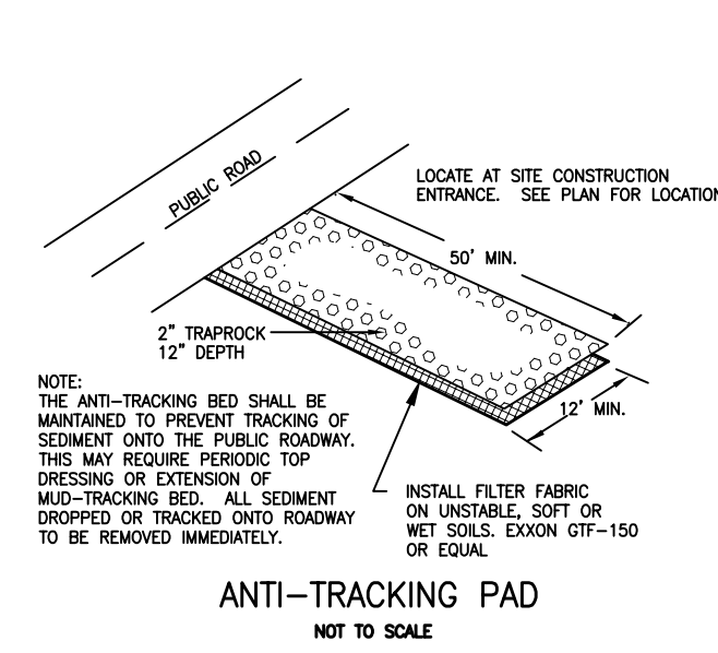
ANTI-TRACKING PAD NOT TO SCALE
