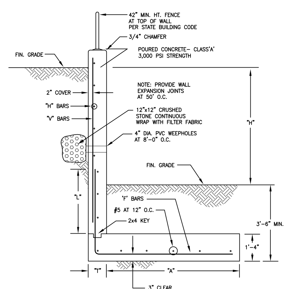
RETAINING WALL NOT TO SCALE
